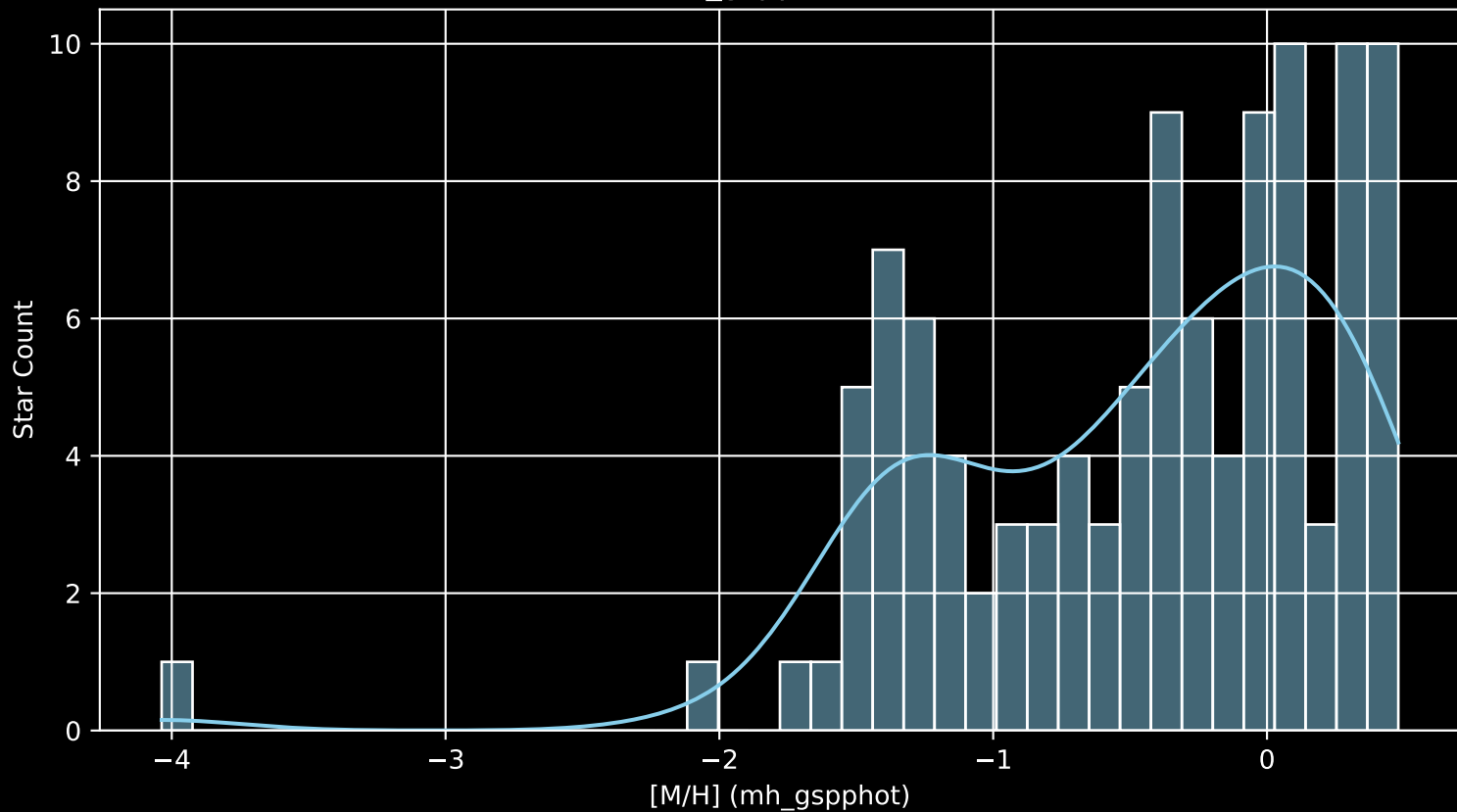
APOGEE DR17 Field: [355+00 [M/H] (mh_gspphot) (n= 107)
