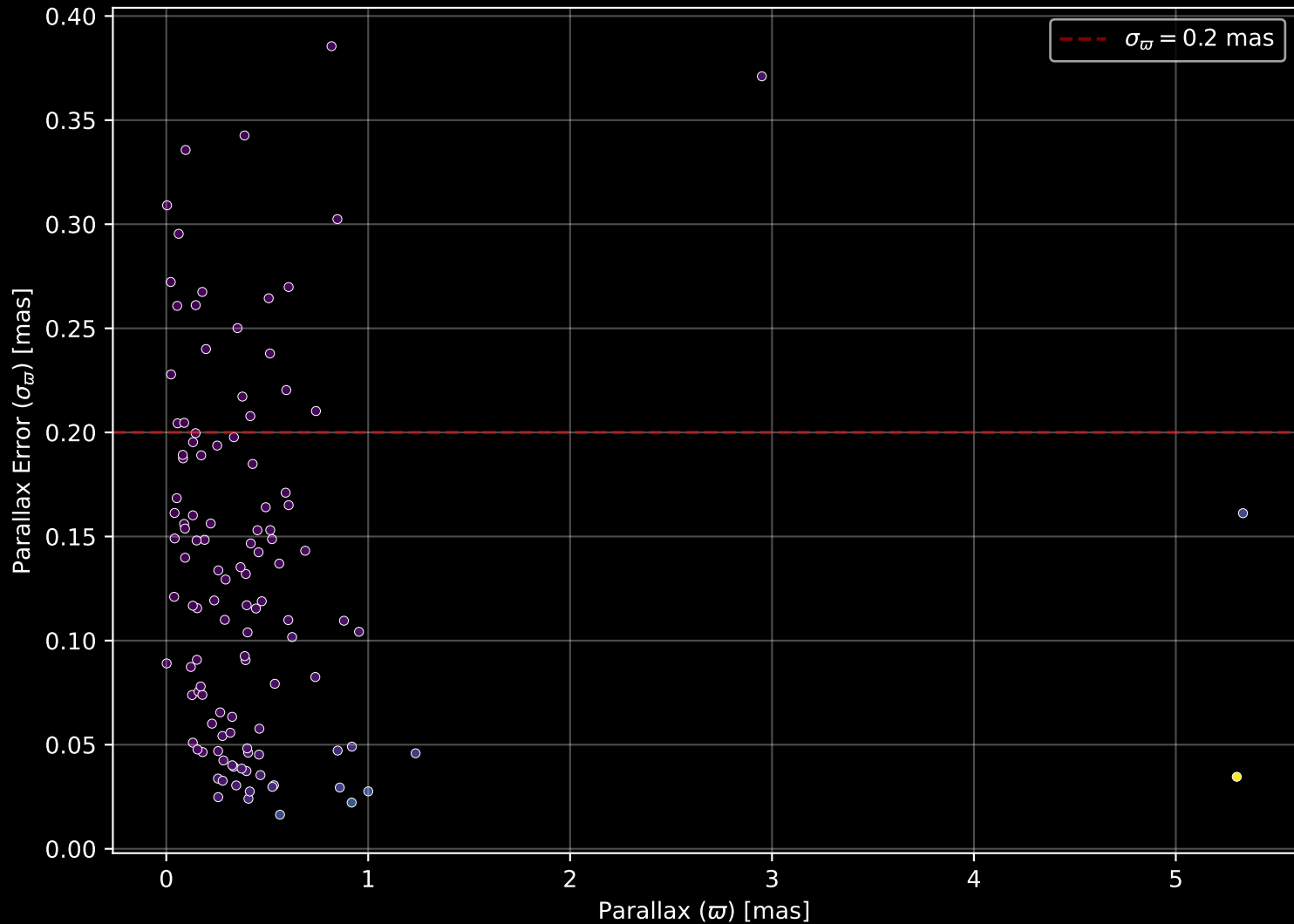
APOGEE DR17 Field: [355+00] Parallax Quality (n= 115)
