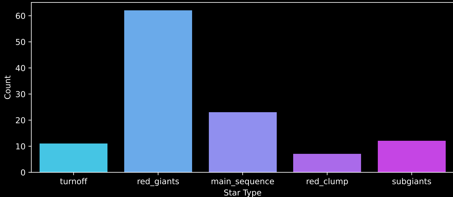
APOGEE DR17 Field: [355+00] Count plot of Star Type
