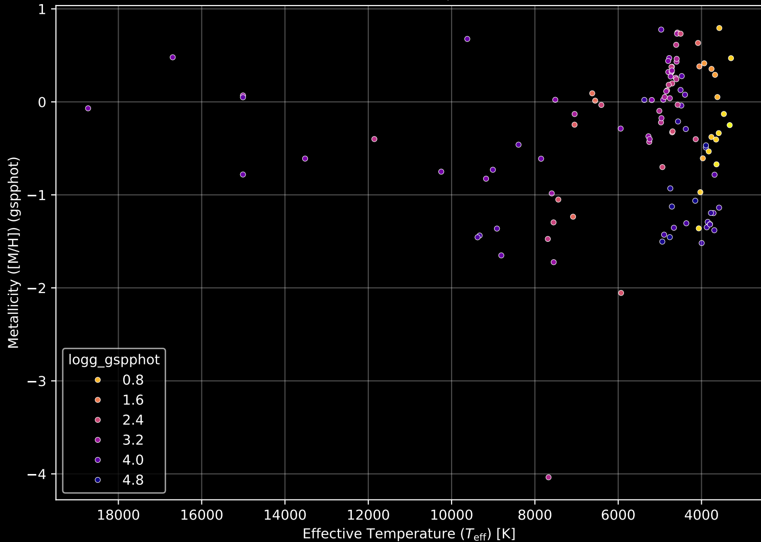
APOGEE DR17 Field: [355+00] Stellar Population Parameters (n= 115)
