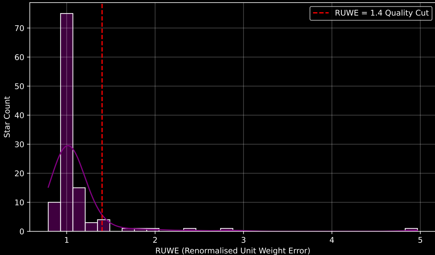
GAPOGEE DR17 Field [355+00] RUWE Distribution (n= 113)
