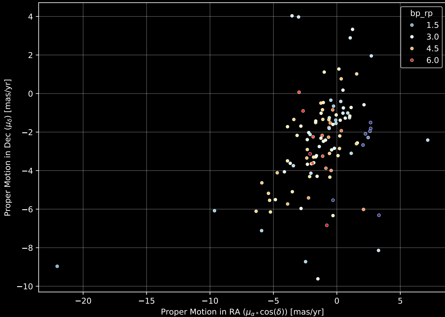
APOGEE DR17 Field: [355+00] Proper Motion Diagram (n= 115)
